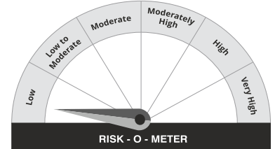
Benchmark Riskometer
