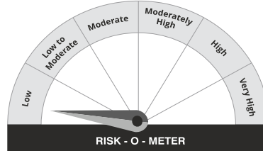
Scheme Riskometer
